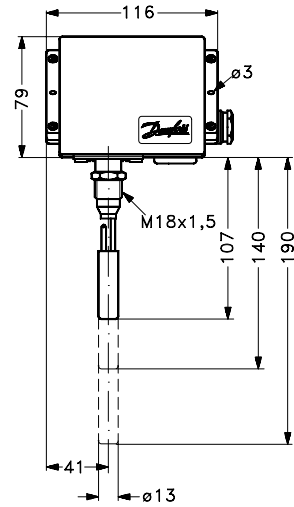
KPS with remote sensor Weight: ca 1.2 kg (incl. 2 m capillary tube)
