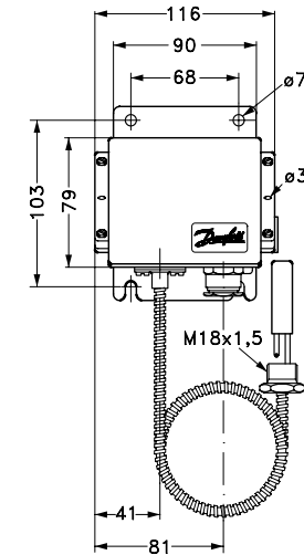
KPS with remote sensor and armoured capillary tube Weight : ca 1.4 kg (incl. 2 m capillary tube)
