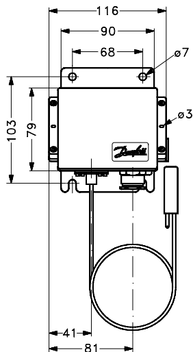
KPS with rigid sensor Weight: ca 1.0 kg
